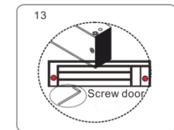
13 Screw door After all the appropriate procedures, the holding force can be maximized. Finally, fix the tamper screw.
