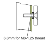
6.8mm for M8-1.25 thread Inside: Drill a hole diameter is 8mm folding the plastic straight pin
