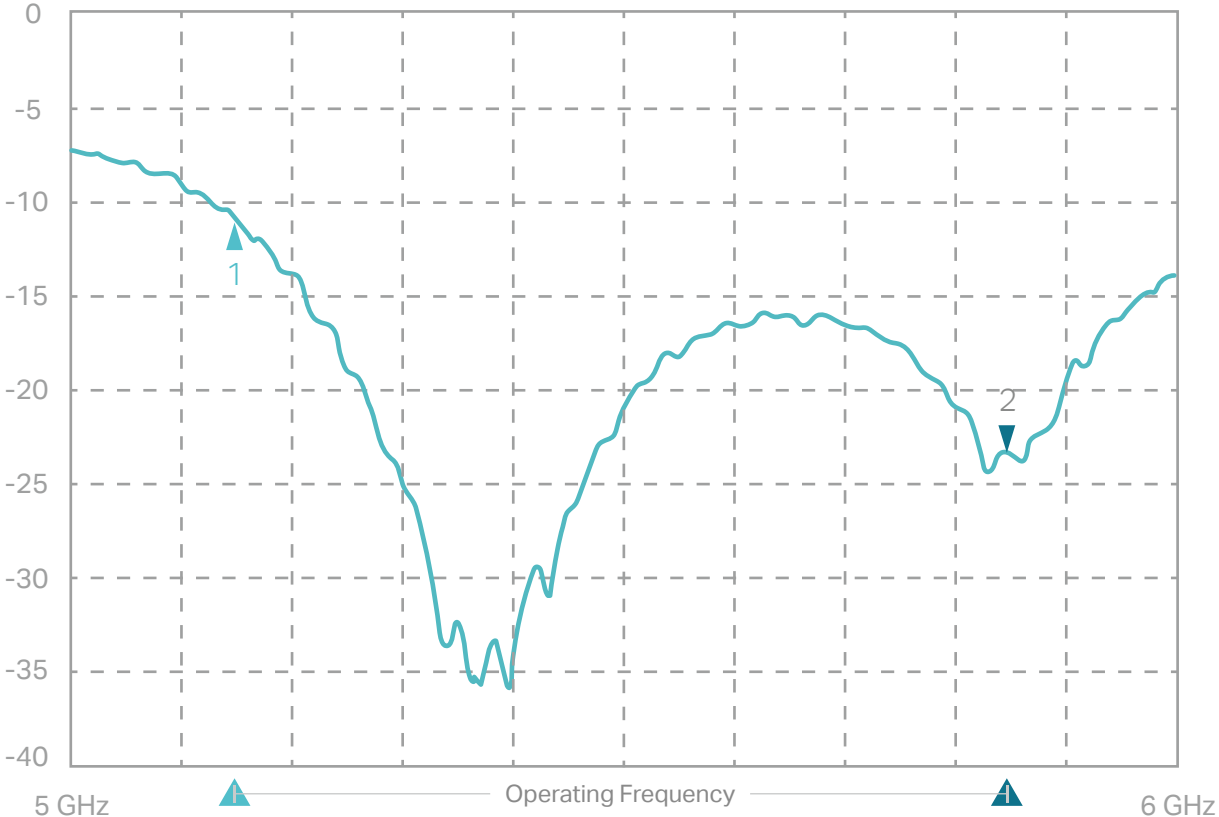
Return Loss
